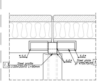
Detail of wall connections – type 10 (top)
