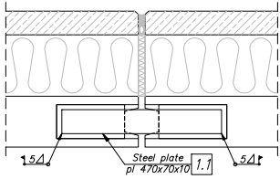
Detail of wall connections – type 7 (top)
