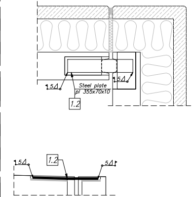
Detail of wall connections – type 9 (top)
