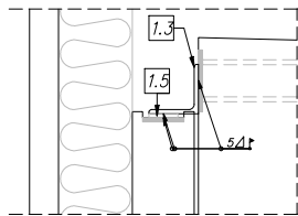
Detail of wall connections – type 12 (top)
