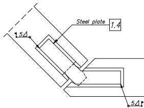
Detail of wall connections – type 12 (top)
